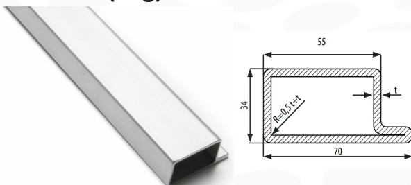
TYPE L (flag) in stock and online.
