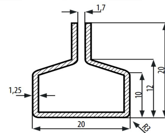
TYPE C On request.
