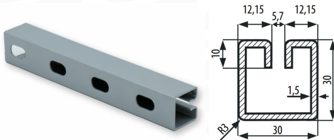
TYPE perforated WG 30X30 in stock and online. Suitable for bottom frame parts (water drainage).
