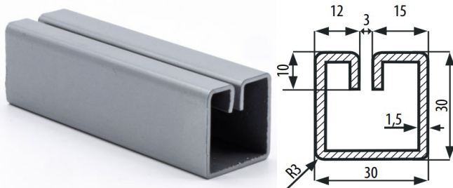
TYPE WE 30X30 in stock and online. Primarily suitable for welded meshes.
