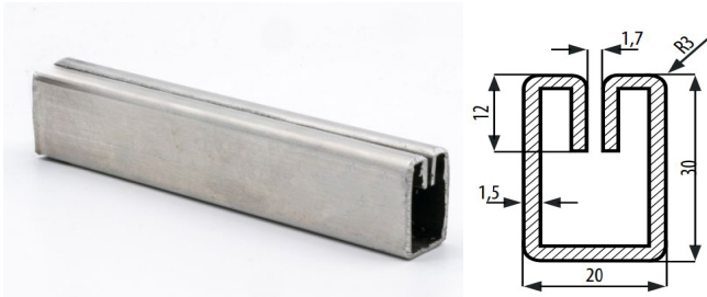
TYPE E in stock and online.
