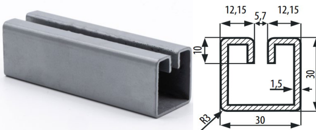
TYPE WG 30X30 in stock and online.
