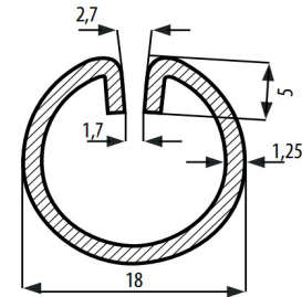
TYPE A On request.
