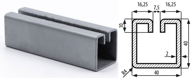
TYPE WG 40X40 in stock and online.
