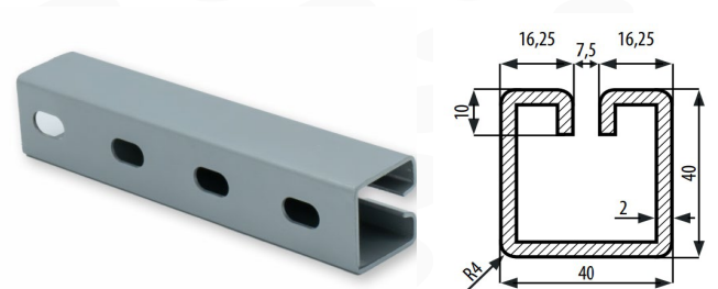
TYPE perforated WG 40X40 in stock and online. Suitable for bottom frame parts (water drainage).
