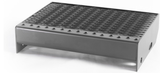
Tread with omnidirectional anti-slip expanded metal, Safe 45 × 13.4/5 mm
